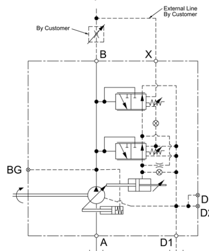
L0 Schematic
